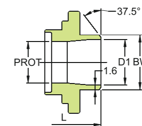
Butt weld end
