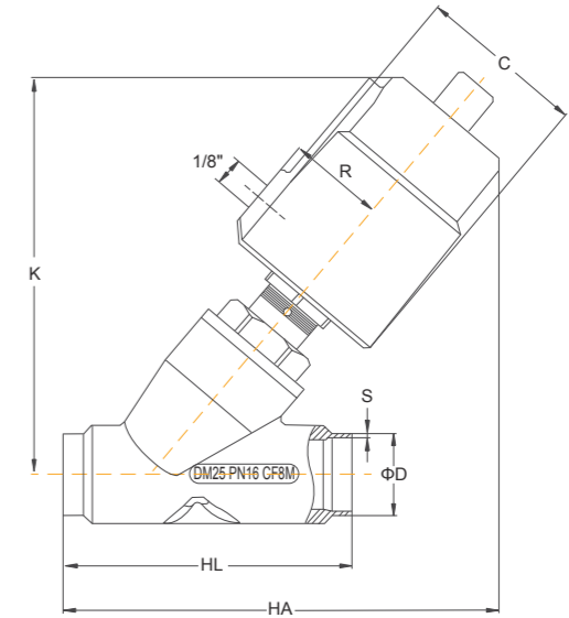
Welded Connection
