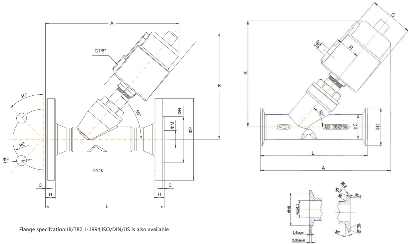
Clamp specification:ISO 2852-1993, According to customer's requirements.
